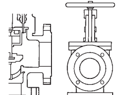
Flanged-End Connection
