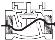
Horizontal-Lift Check Valve
